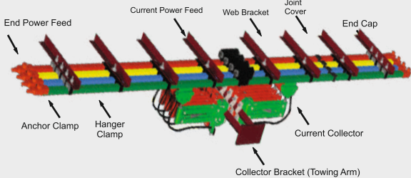
DSL Shrouded Busbar System
