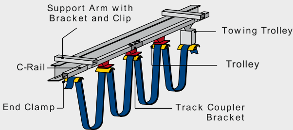
Festoon System ( C-Rail )
